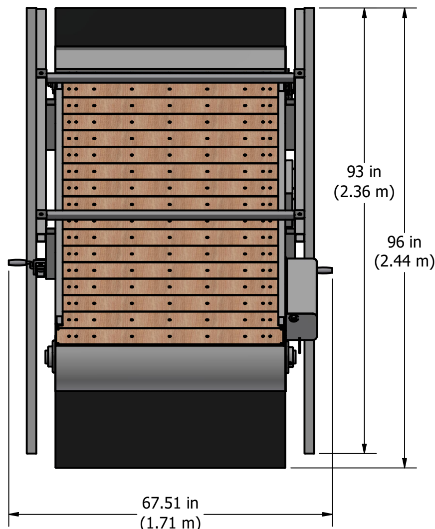
Top View
