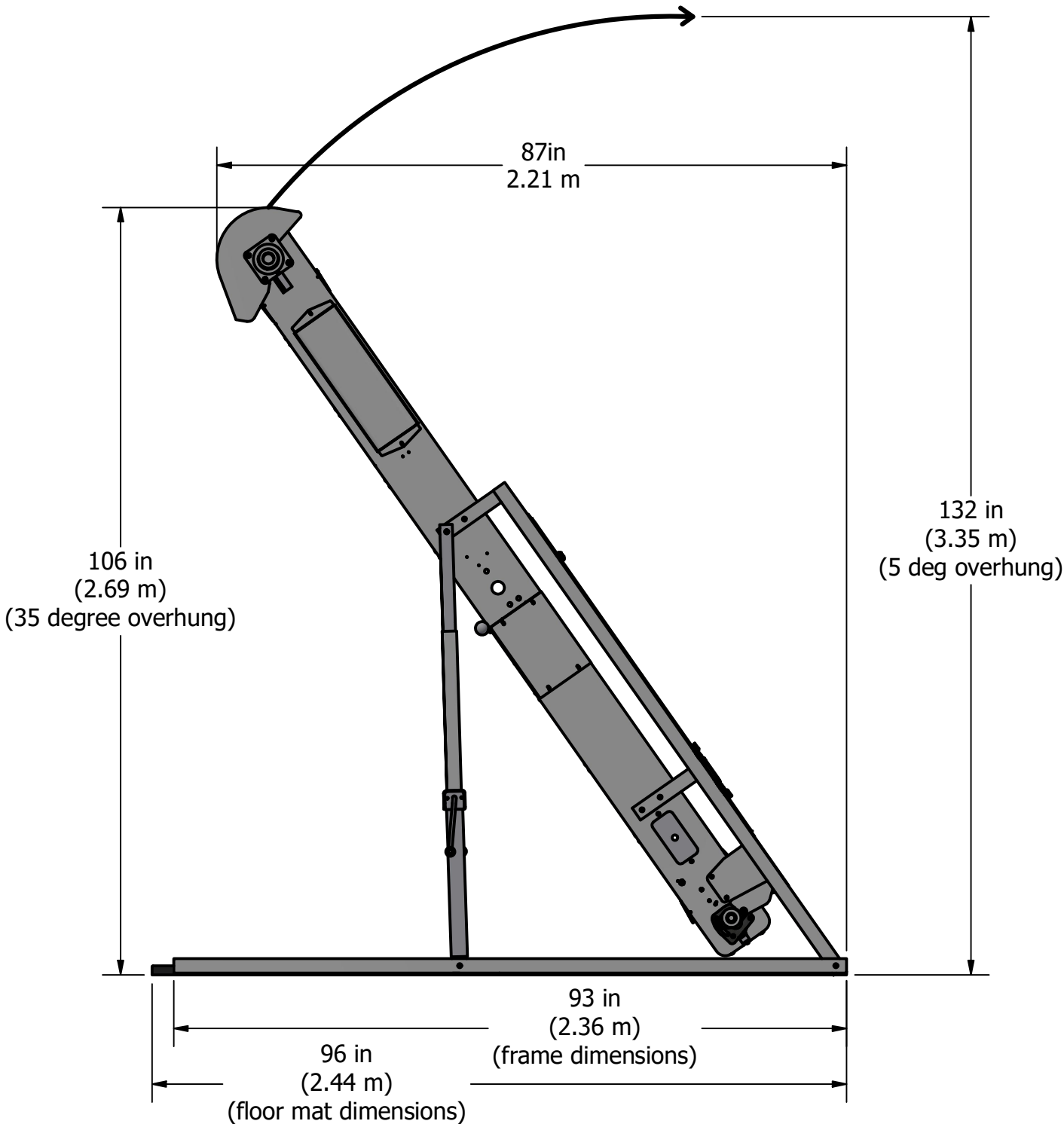
Side View
