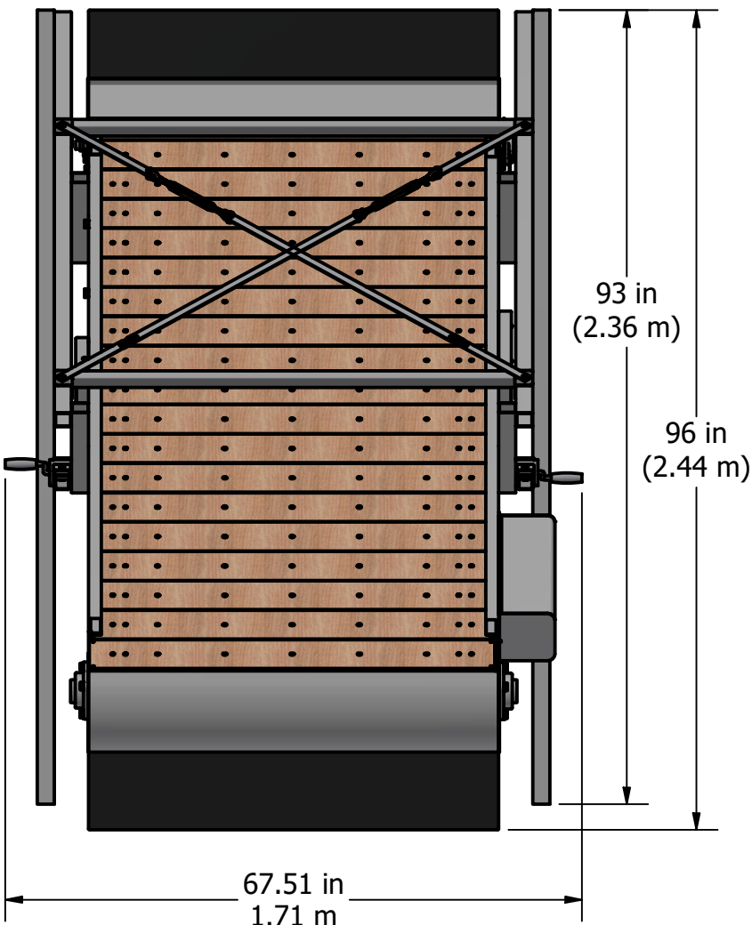
Top View
