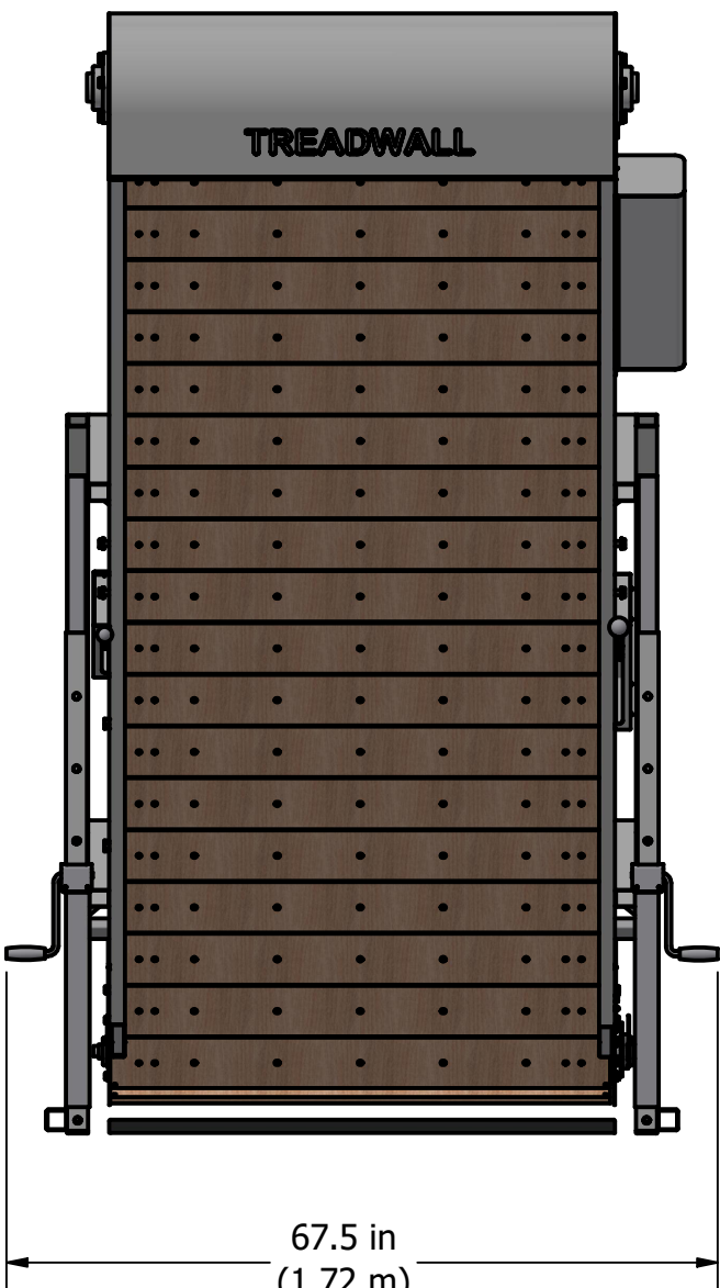
Front View
