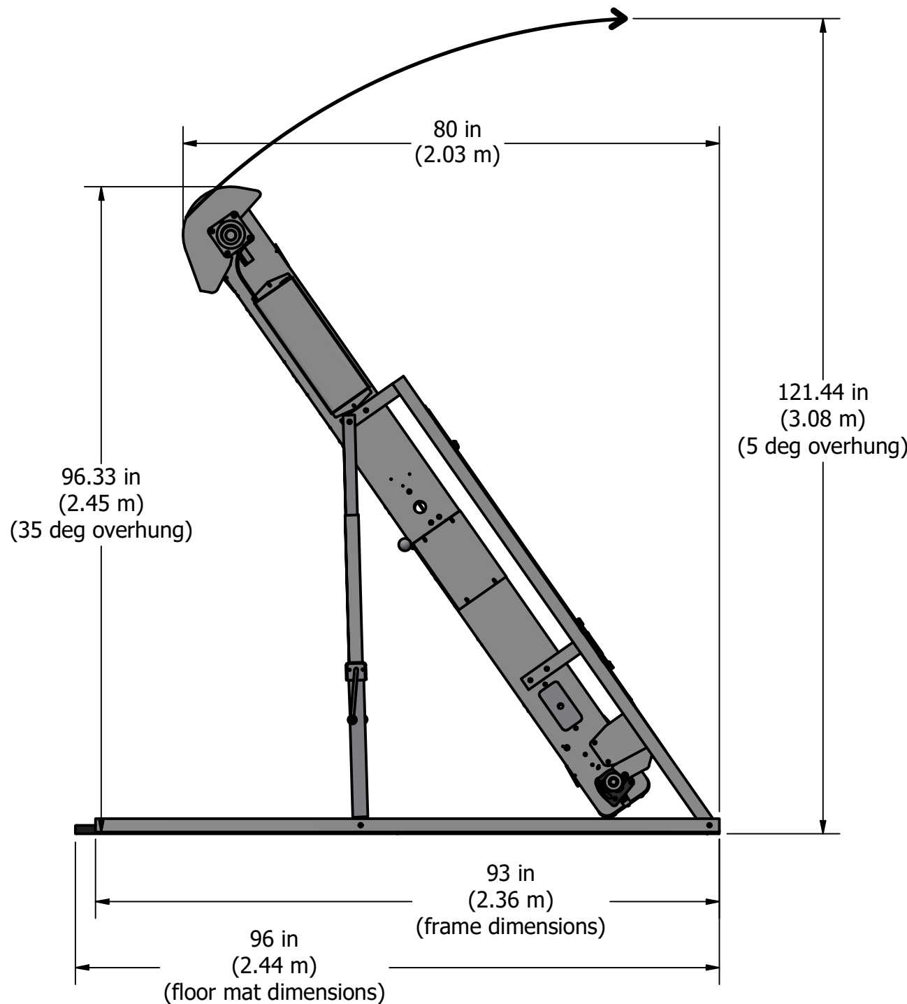
Side View
